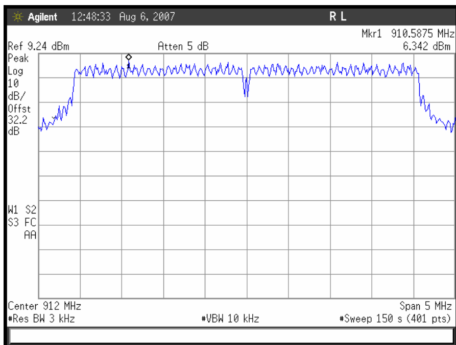
Plot 35. 802.11/g – 912MHz Low Ch Peak Power Spectral Density, 5MHz
