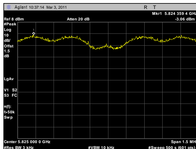
Plot 29. Peak Spectral Density, High Channel
