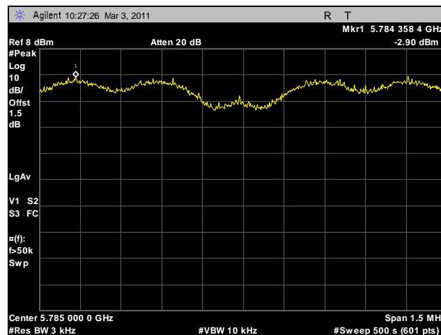
Plot 28. Peak Spectral Density, Mid Channel
