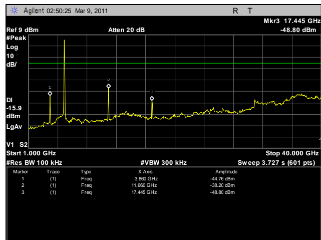
Plot 24. Conducted Spurious Emissions, High Channel, 1 GHz – 40 GHz
