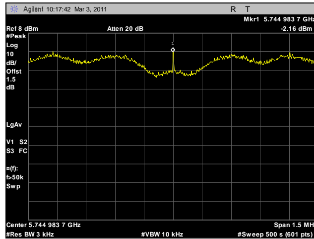
Plot 27. Peak Spectral Density, Low Channel
