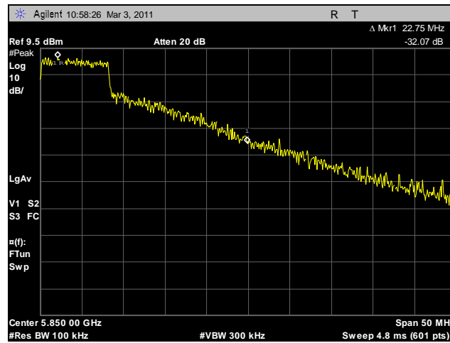
Plot 26. Conducted Band Edge, High Channel
