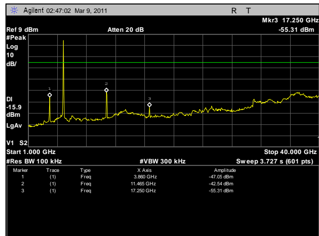
Plot 20. Conducted Spurious Emissions, Low Channel, 1 GHz – 40 GHz
