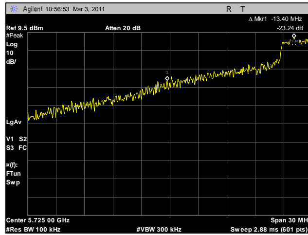
Plot 25. Conducted Band Edge, Low Channel
