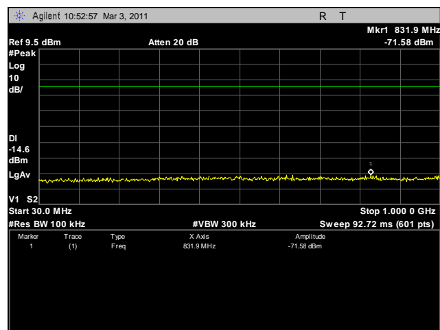
Plot 21. Conducted Spurious Emissions, Mid Channel, 30 MHz – 1 GHz
