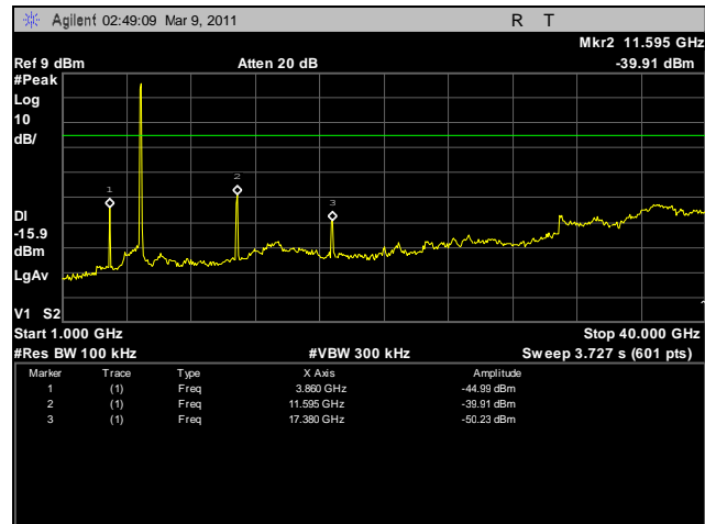
Plot 22. Conducted Spurious Emissions, Mid Channel, 1 GHz – 40 GHz
