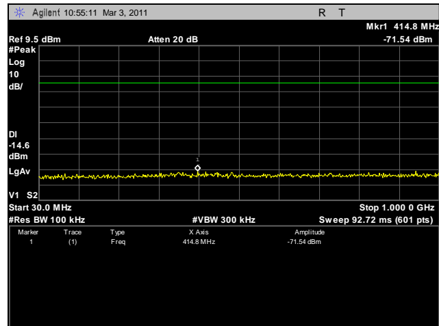
Plot 19. Conducted Spurious Emissions, Low Channel, 30 MHz – 1 GHz
