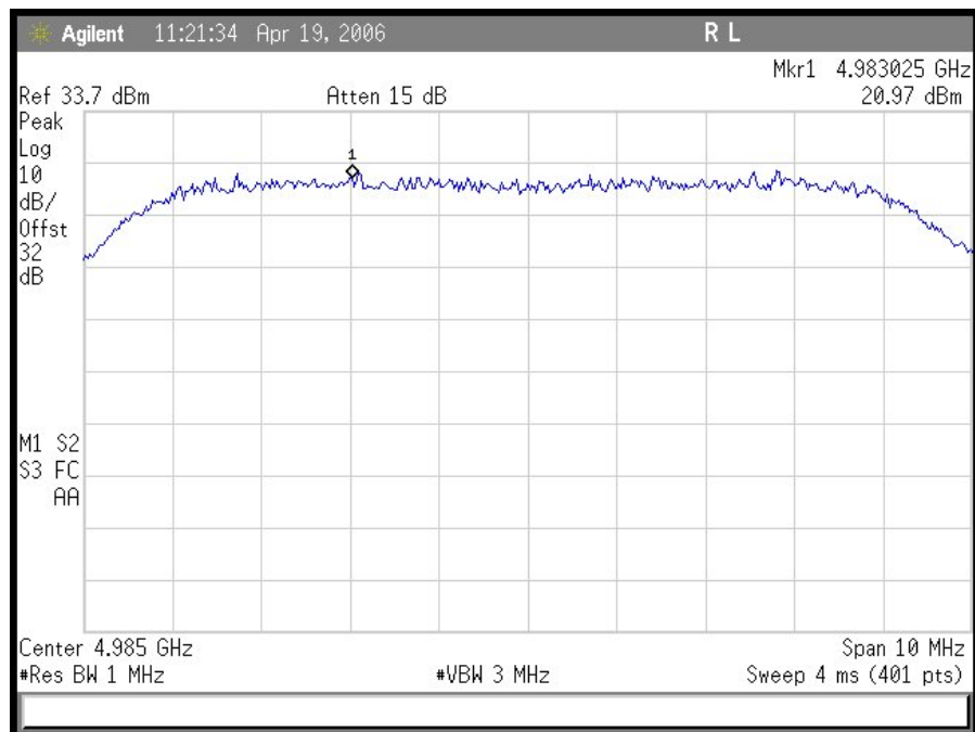
Plot 6. PSD 10 MHz High Ch
