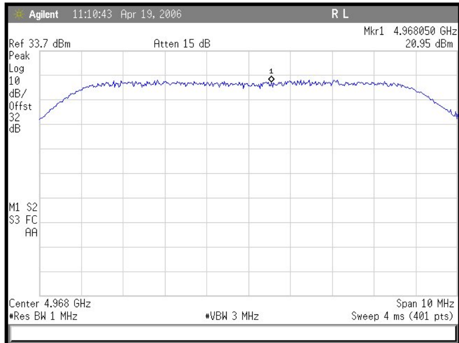
Plot 5. PSD 10 MHz Mid Ch
