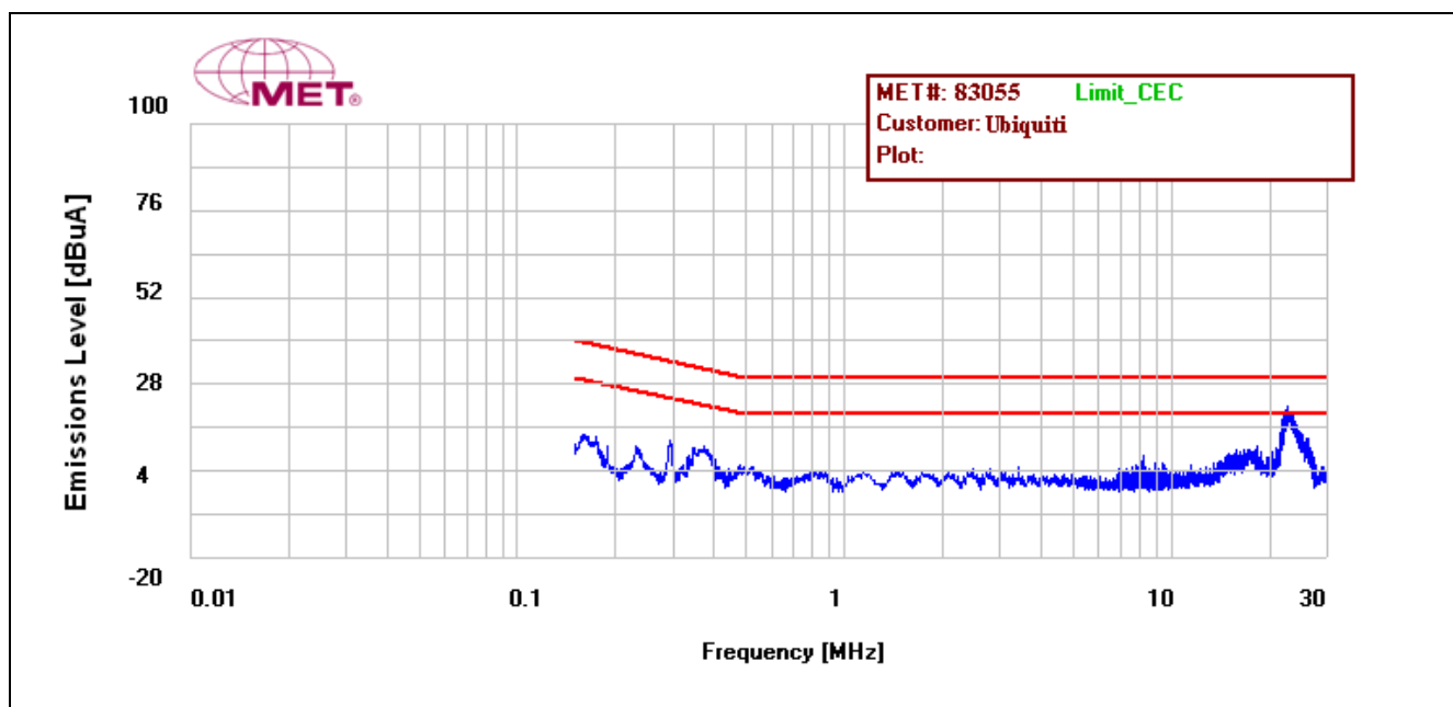
Plot 3. Conducted Emission Limits for Telecommunications Ports, LAN Plot
