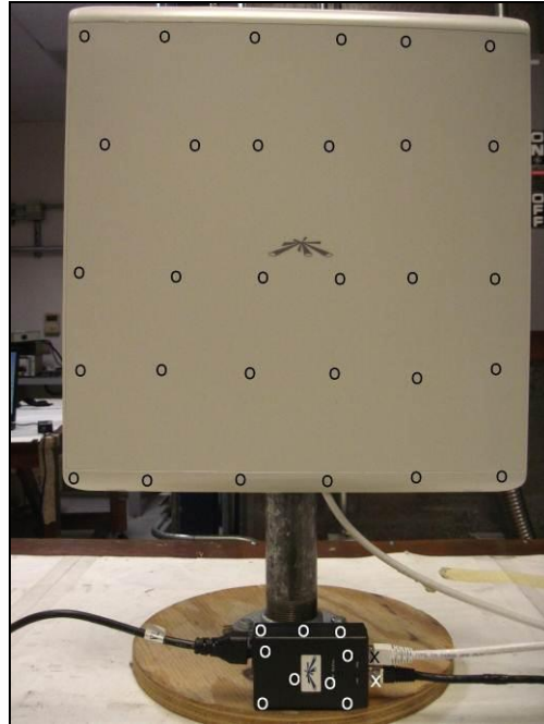
Photograph 8. ESD, Test Points, Front View
