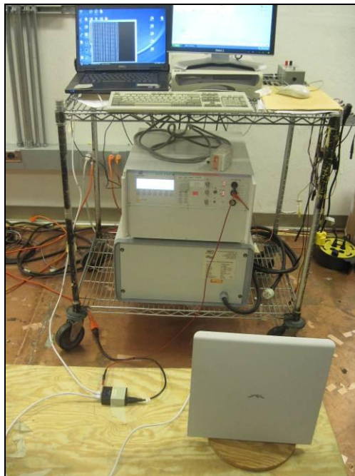
Photograph 17. Surges, Test Setup, I/O Mode
