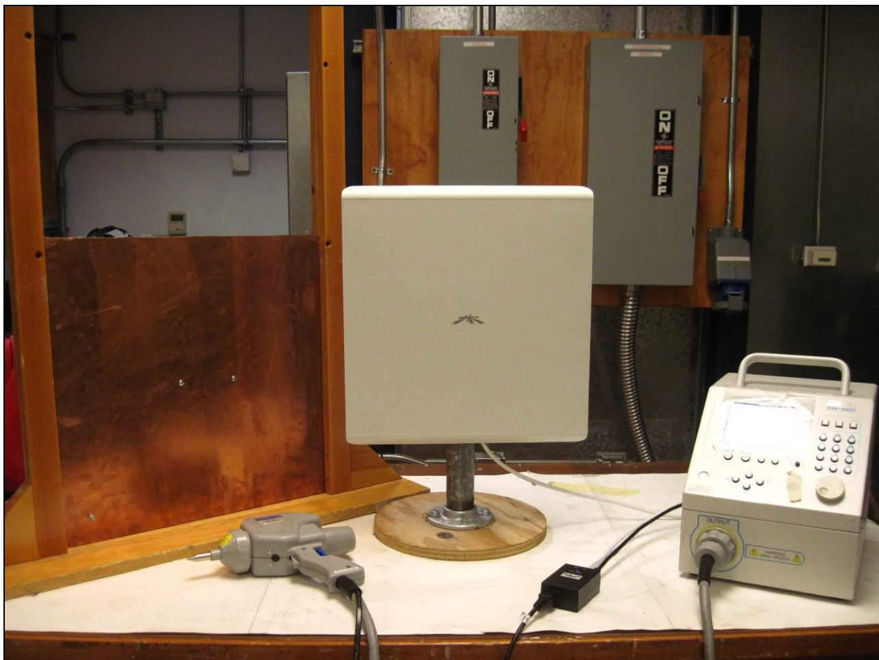
Photograph 10. Electrostatic Discharge, Test Setup
