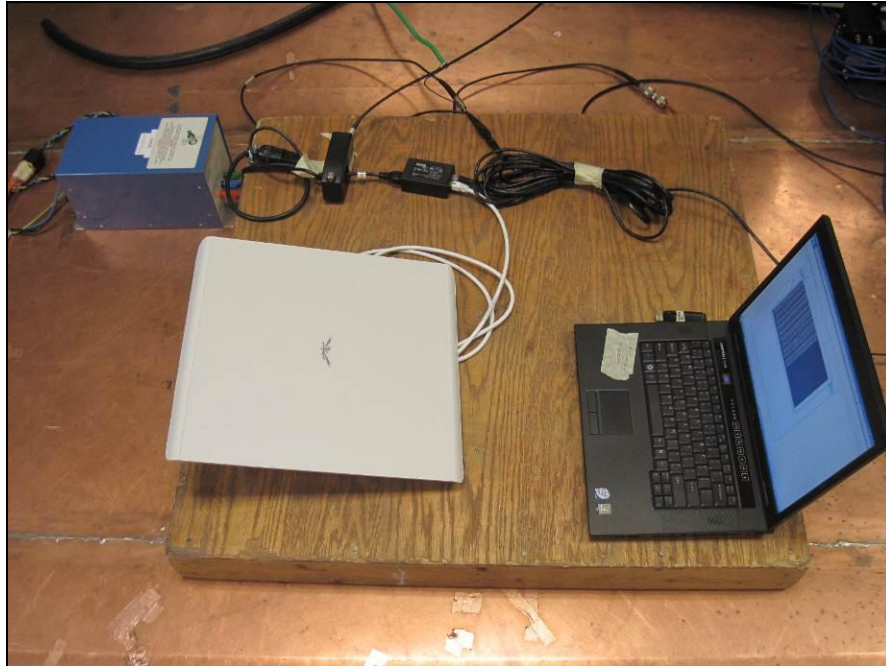
Photograph 13. Radio Frequency, Common Mode, Test Setup, AC Mode
