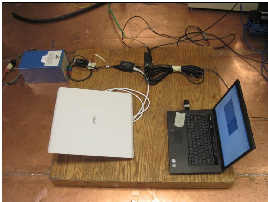
Photograph 14. Radio Frequency, Common Mode, Test Setup, I/O Mode
