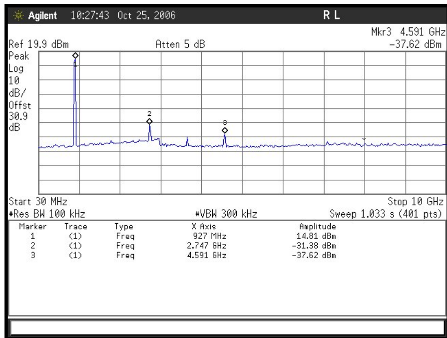
Plot 13. 802.11/b – Mid Channel Conducted Emissions 30MHz – 10GHz (OFDM – 10MHz)
