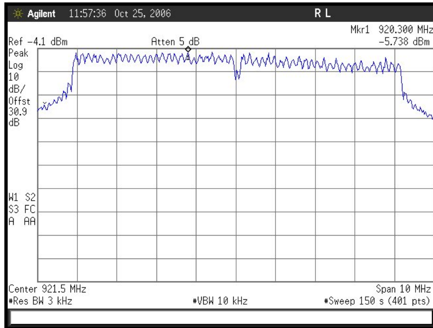
Plot 33. 802.11/g – High Ch Peak Power Spectral Density – OFDM 10MHz
