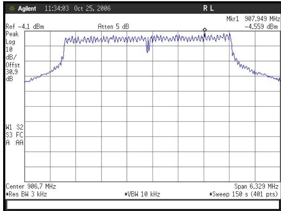
Plot 27. 802.11/g – Low Ch Peak Power Spectral Density – OFMD 5MHz
