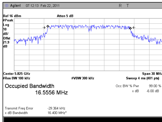
Plot 10. 6 dB Occupied Bandwidth, High Channel
