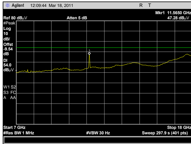
Plot 23. Radiated Harmonics, Mid Channel, Average
