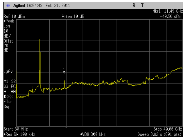
Plot 27. Conducted Spurious Emissions, Low Channel, 30 MHz – 40 GHz
