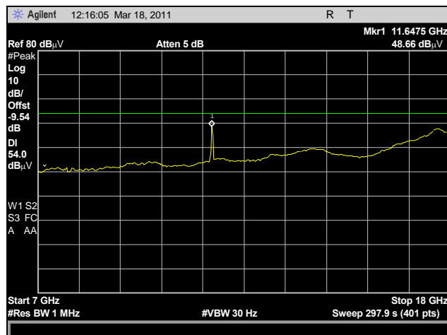
Plot 25. Radiated Harmonics, High Channel, Average
