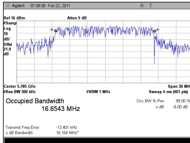
Plot 12. 99% Occupied Bandwidth, Mid Channel
