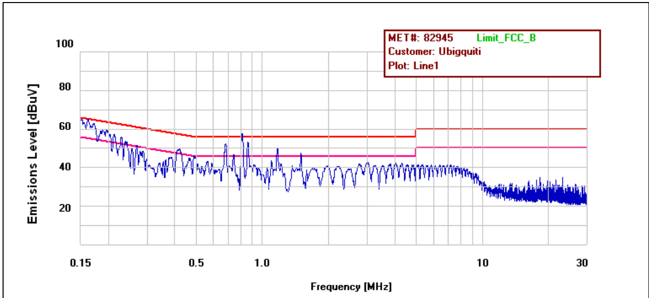
Plot 6. Conducted Emissions, 15.207(a), Phase Line
