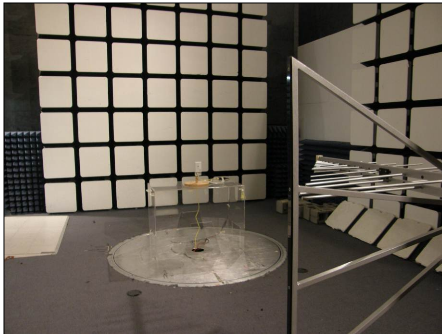
Photograph 7. Radiated Spurious Emissions, Test Setup, 30 MHz – 1 GHz
