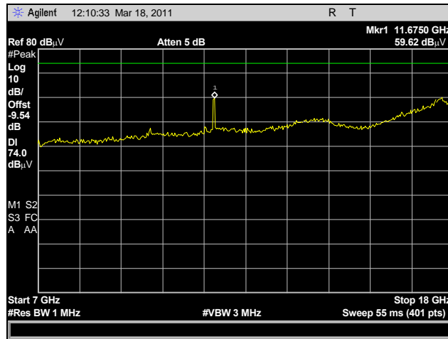
Plot 26. Radiated Harmonics, High Channel, Peak
