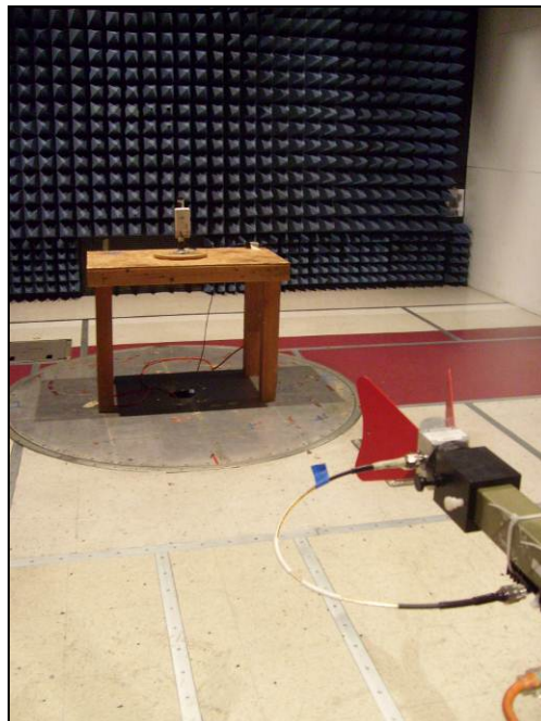
Photograph 4. Radiated Emissions, Test Setup, 1 GHz – 10 GHz
