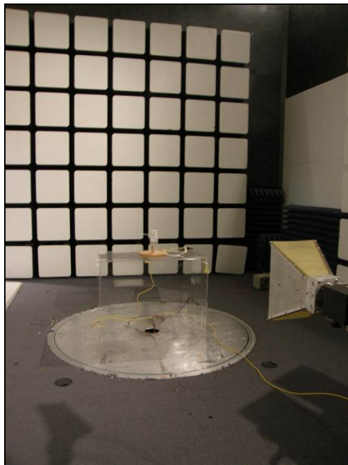
Photograph 8. Radiated Spurious Emissions, Test Setup, 1 GHz – 18 GHz
