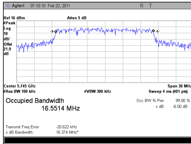
Plot 8. 6 dB Occupied Bandwidth, Low Channel
