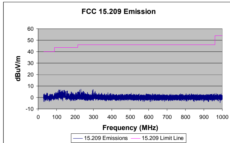
Plot 17. Radiated Spurious Emissions, Mid Channel, 30 MHz – 1 GHz
