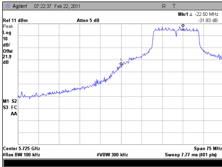
Plot 30. Conducted Band Edge, Low
