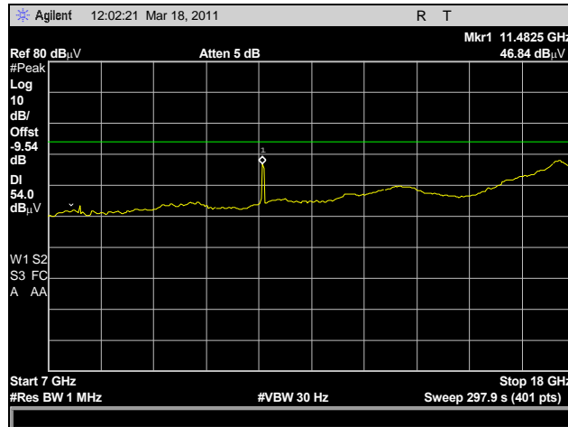
Plot 21. Radiated Harmonics, Low Channel, Average
