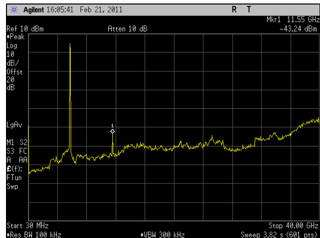
Plot 28. Conducted Spurious Emissions, Mid Channel, 30 MHz – 40 GHz
