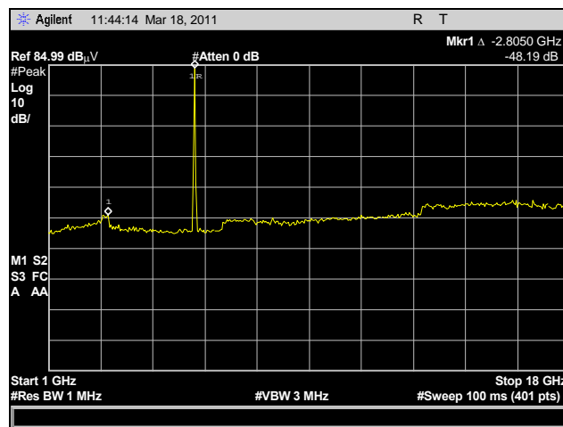
Plot 18. Radiated Spurious Emissions, Low Channel, 1 GHz – 18 GHz
