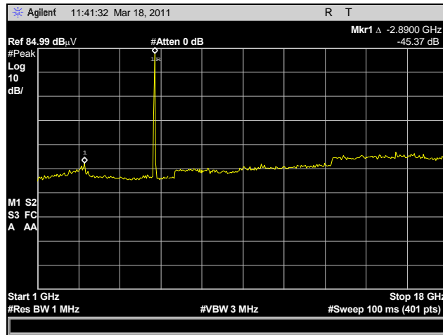
Plot 20. Radiated Spurious Emissions, High Channel, 1 GHz – 18 GHz
