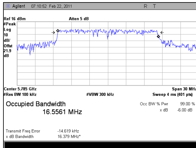
Plot 9. 6 dB Occupied Bandwidth, Mid Channel
