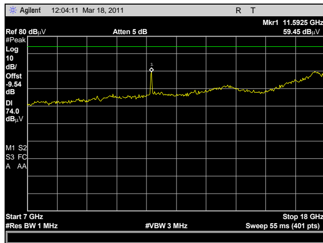
Plot 24. Radiated Harmonics, Mid Channel, Peak
