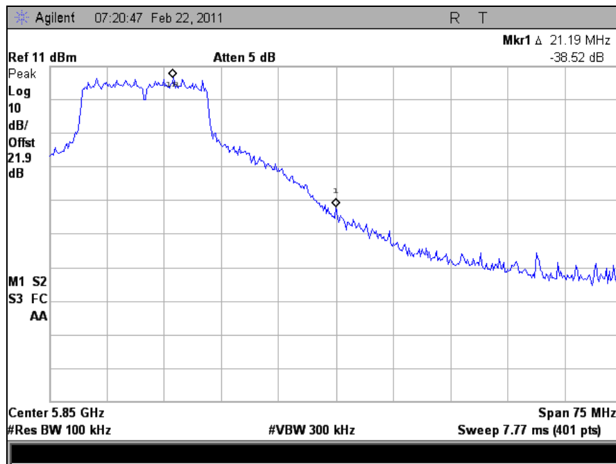
Plot 31. Conducted Band Edge, High
