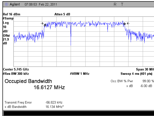
Plot 11. 99% Occupied Bandwidth, Low Channel
