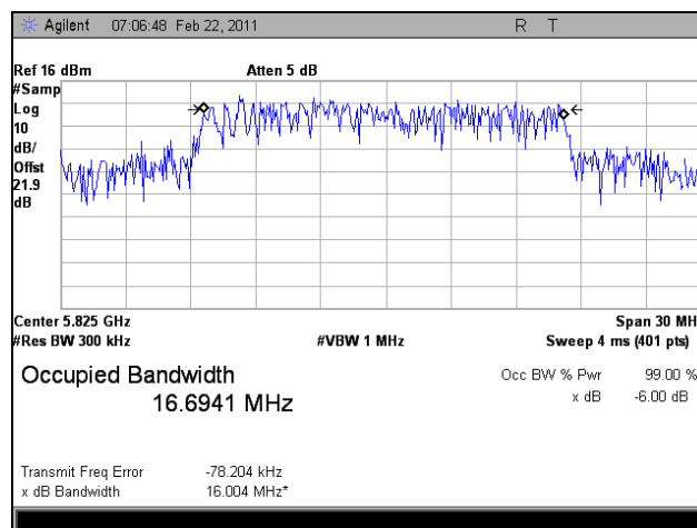
Plot 13. 99% Occupied Bandwidth, High Channel
