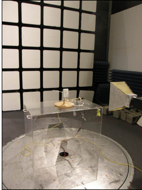
Photograph 6. Radiated Harmonics, Test Setup, 1m Distance
