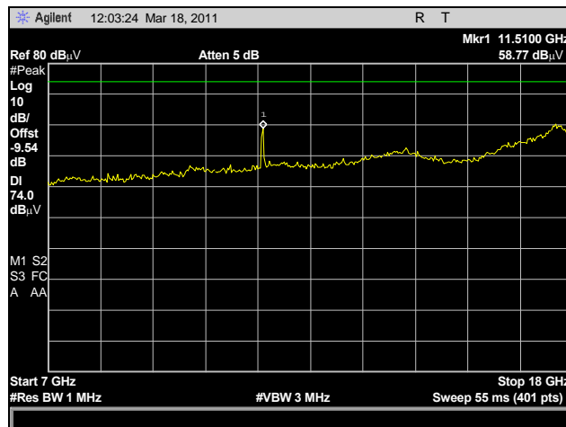
Plot 22. Radiated Harmonics, Low Channel, Peak
