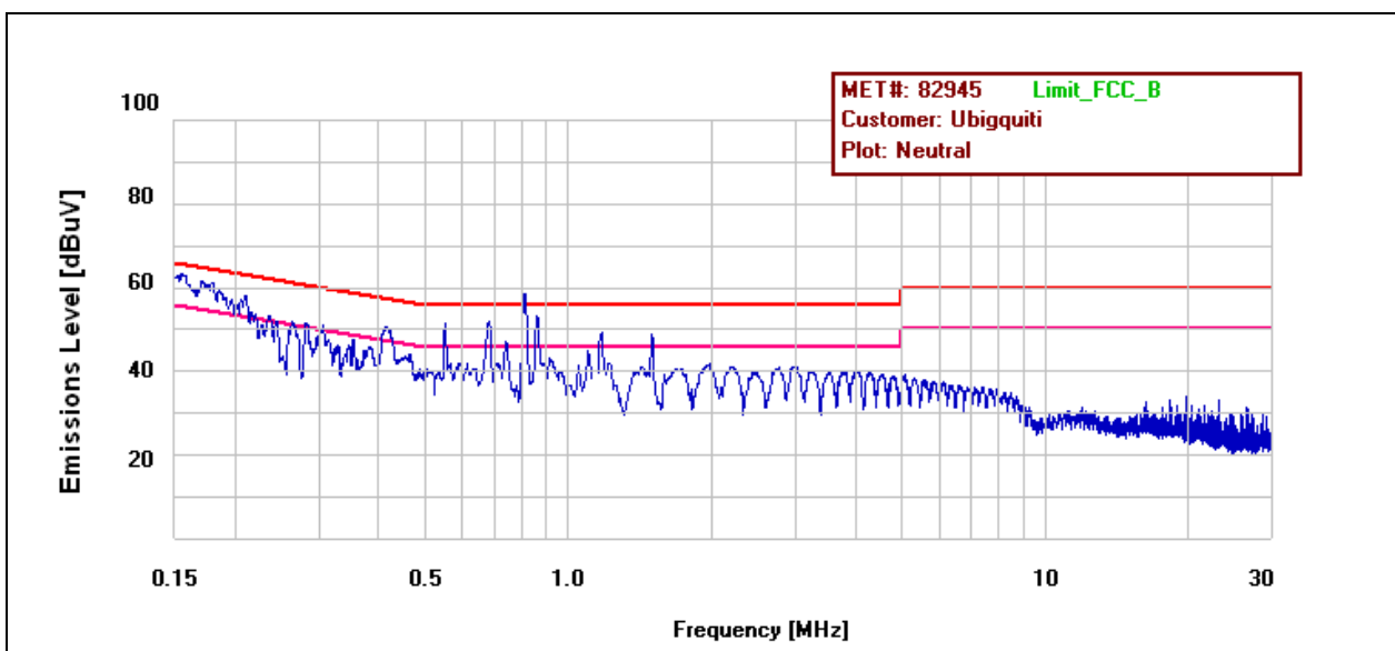
Plot 7. Conducted Emissions, 15.207(a), Neutral Line
